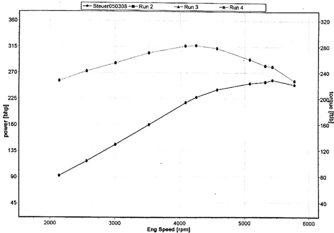
Power Curve
