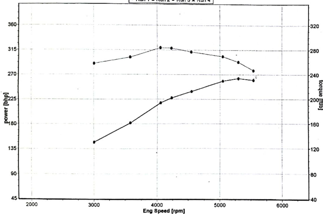
Power Curve
